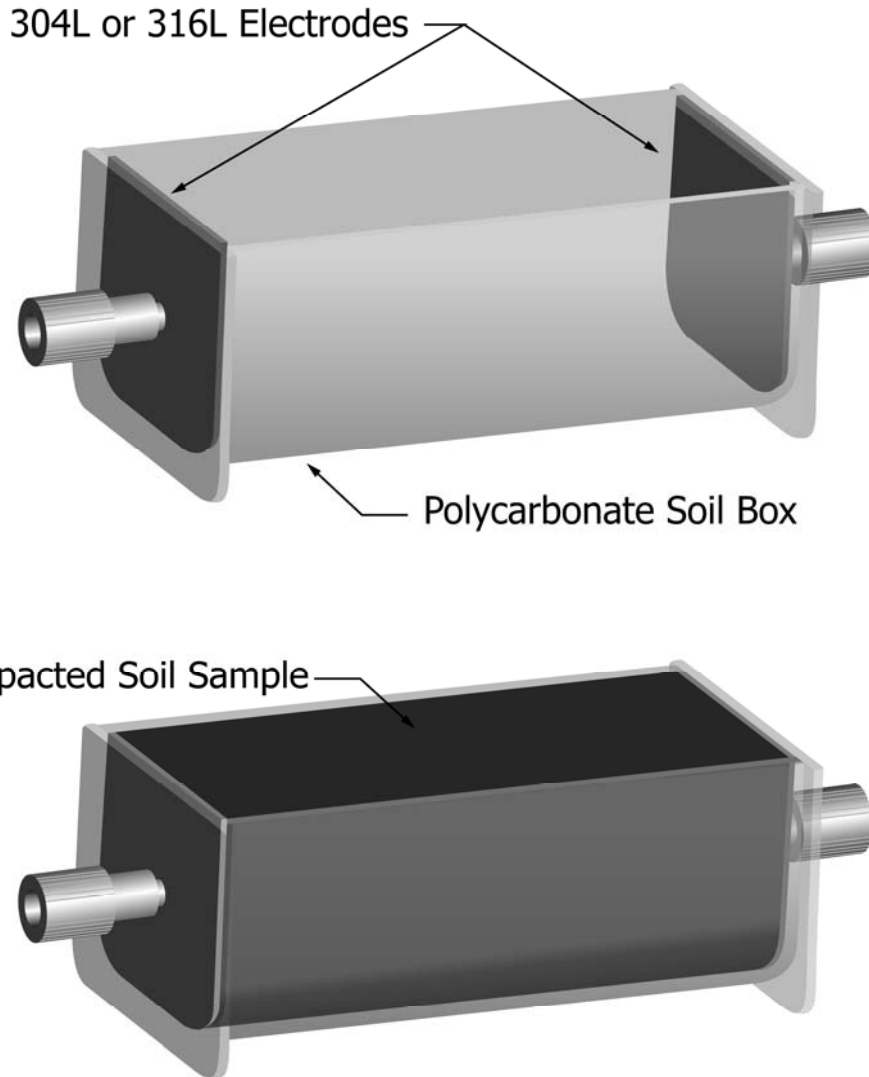
FIG. 2 Typical Two-Electrode Soil Box (Empty and Full)
